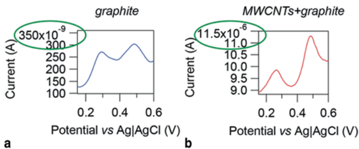
Fig. 6.1 Zoom of oxidation peaks of a metabolite of medical interest, bilirubin ( 150 \mu\text{M} in 0.01 \text{ M} phosphate buffer solution, \text{pH } 7.4 ) at bare a and nanostructured b electrodes. The green circles underline the increase of orders of magnitude of the peak currents at carbon nanostructured electrodes
