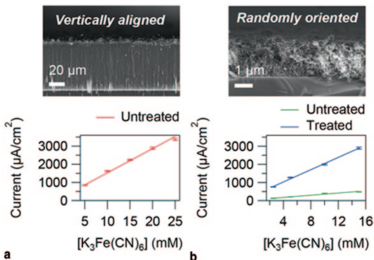
Fig. 6.3 Calibration curves obtained from the detection of [\text{Fe}(\text{CN})_6]^{3+/2+} at vertically aligned a and randomly oriented b MWCNTs. Results before (in green) and after (in blue) a chemical activation are shown for randomly oriented CNTs [5]
