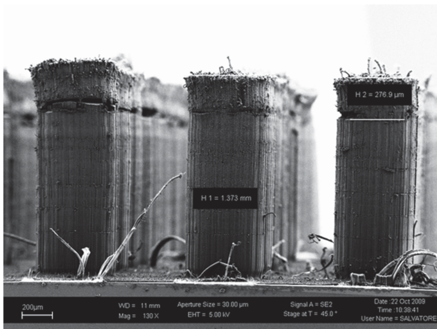
Fig. 6.9 Free standing vertically aligned multi wall carbon nanotube
