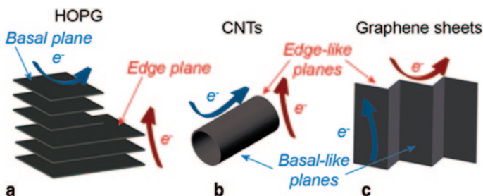
Fig. 6.2 Structure of a HOPG, b CNTs and c graphene sheets. The edge-plane-like sites responsible of a faster electron transfer rate are shown
