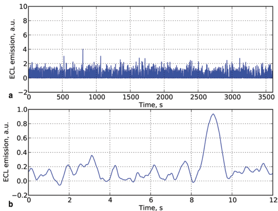
Fig. 6.10 CNT emitted raw signal data a and processed signal resulting after gated averaging b Scan rate: 500 \text{ mV s}^{-1}
